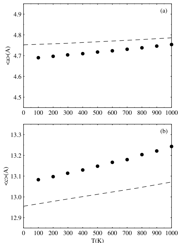
Figure 5. Lattice lengths of \alpha - \text{Al}_2\text{O}_3 hexagonal structural unit cell vs temperature at P = 0 GPa: (a) \langle a \rangle , (b) \langle c \rangle . Dots and line denote the current results and fitting of experimental results of [20], respectively.
