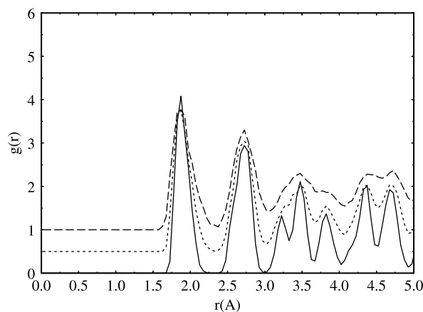
Figure 6. Pair distribution function of \alpha - \text{Al}_2\text{O}_3 at P = 0 GPa and different temperature T . Solid, dot and dish lines denote T = 298 K [ g(r) ], 600 K [ g(r) + 0.5 ] and 1000 K [ g(r) + 1.0 ], respectively.
