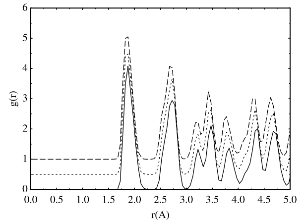
Figure 4. Pair distribution function of \alpha - \text{Al}_2\text{O}_3 at T = 298 K and different hydrostatic pressure P . Solid, dot and dash lines denote P = 0 GPa [ g(r) ], 5 GPa [ g(r) + 0.5 ] and 10 GPa [ g(r) + 1.0 ], respectively.
