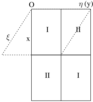
Figure 1. A plane schematic for combining two hexagonal unit cells to a rectangular one through transformation of the body coordinates ( \xi, \eta, \zeta ) to Cartesian coordinates ( x, y, z ). Dot and solid lines denote the hexagonal and the rectangular unit cells, respectively.
